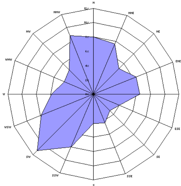
Figure E.7.8. Wind rose displaying wind direction frequency.
