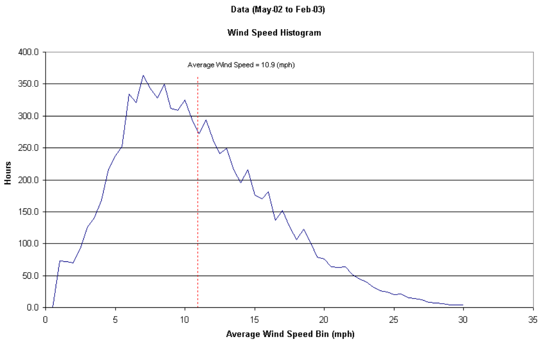
Figure E.7.4. Wind speed frequency over the year by # of hours.
