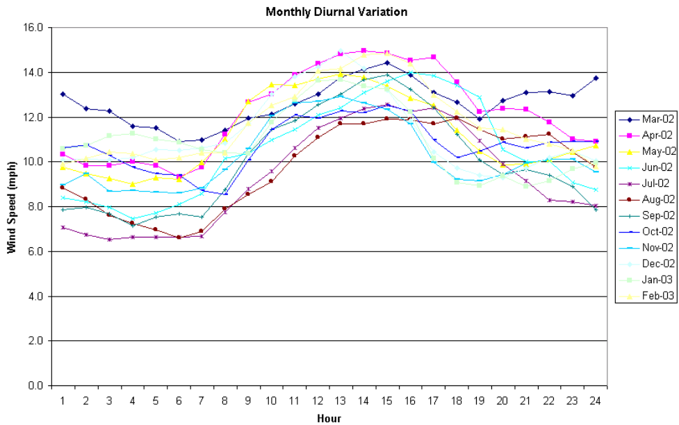
Figure E.7.3. Average hourly wind speeds for each month.
