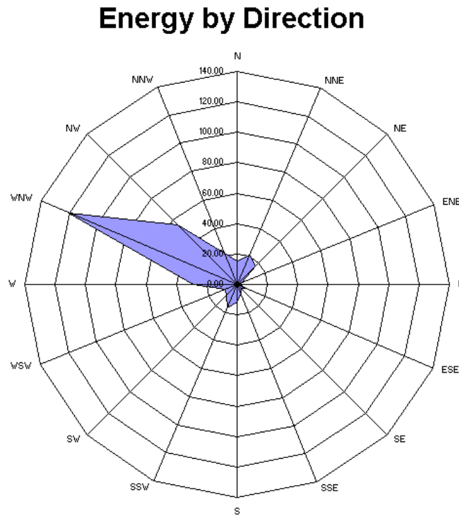
Figure 9. Energy wind rose with units in kWh/m 2 .
